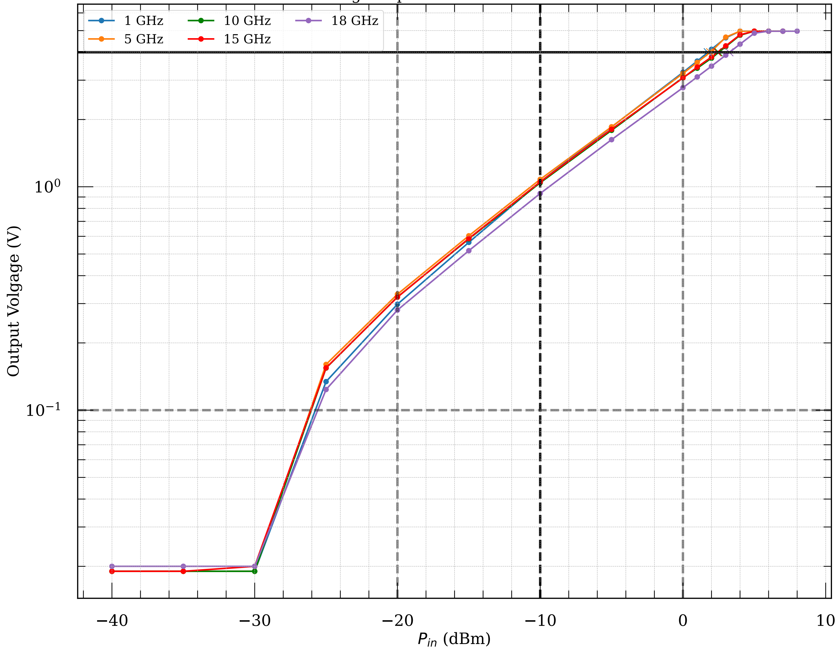
Measured voltage-to-power curve of detector module079
